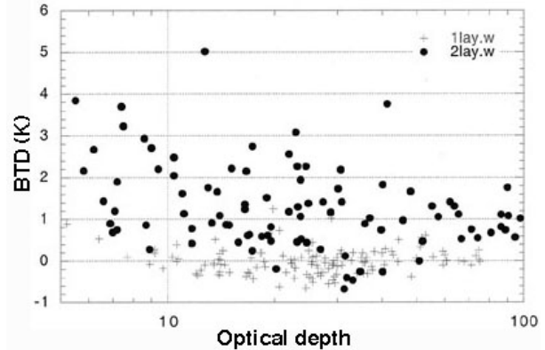
Fig. 3. Variation of mean BT in 0.3° box from GOES-8 for 1 and 2-layered clouds identified as liquid water.
